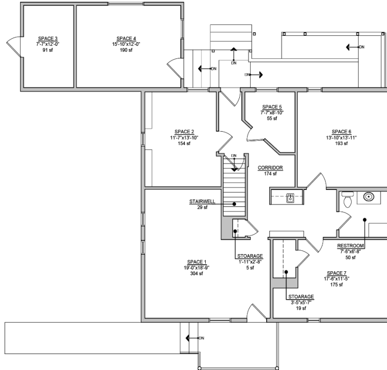
1st Floor ±1,629 SF
